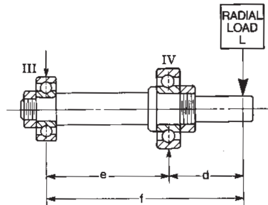
Fig. 4 Overhung Mounting
