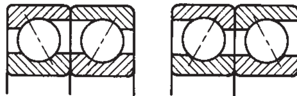
Face-to-face Back-to-back Figure 4 Angular contact ball bearings pair mounting arrangements.
